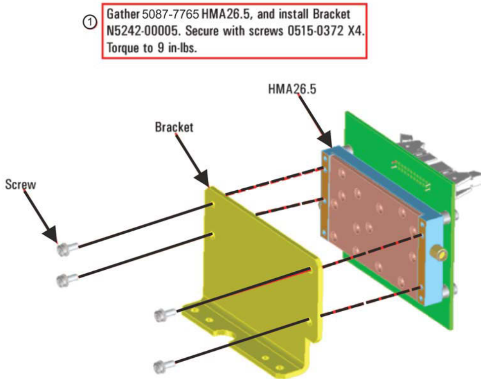
Figure 2 A21 LO Multiplier/Amplifier (HMA26.5) Assembly
