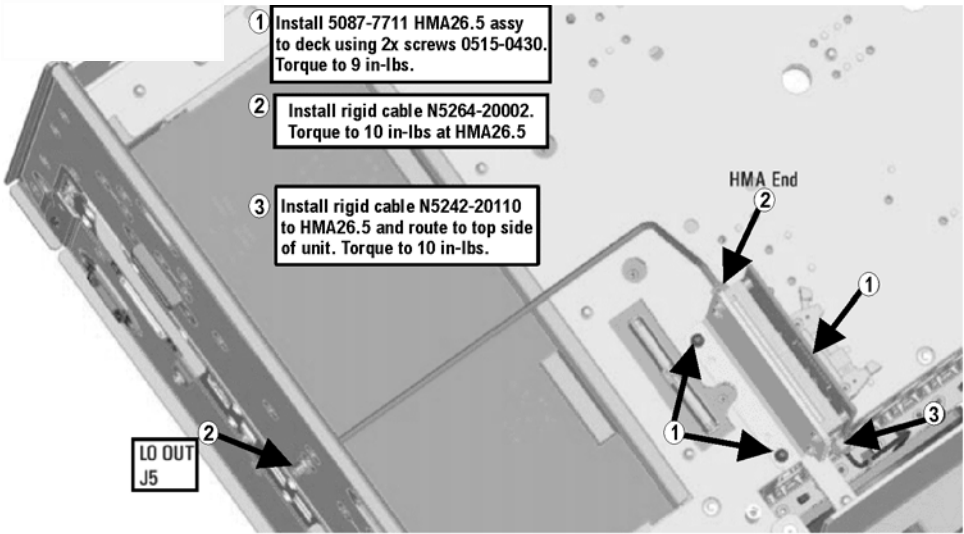
Figure 3 A21 LO Multiplier/Amplifier (HMA26.5) Installation
