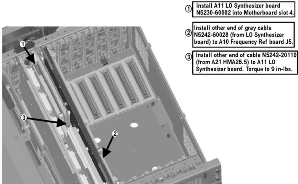
Figure 5 A11 13.5 GHz LO Synthesizer Board Installation
